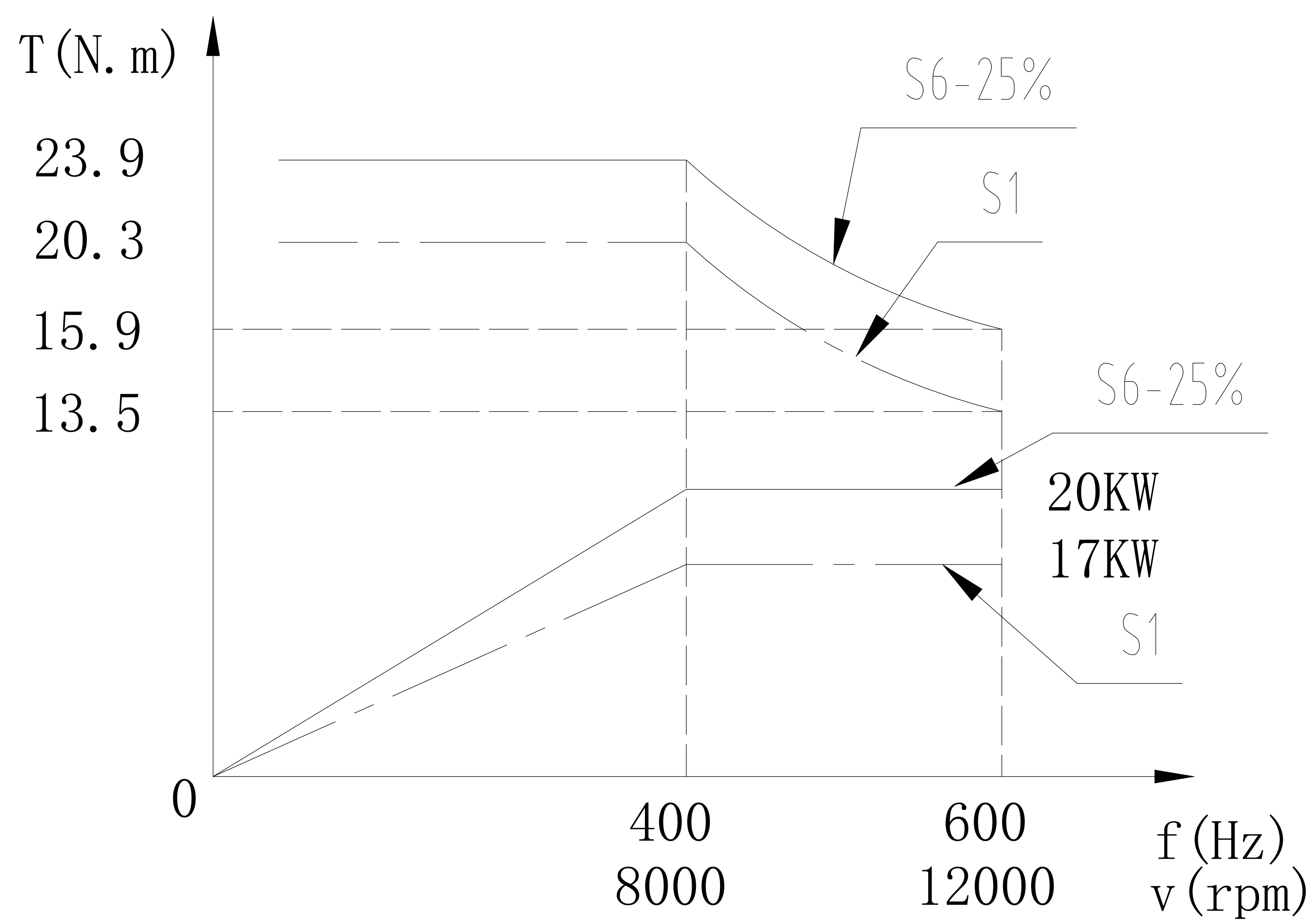
Torque/P.f Curve
